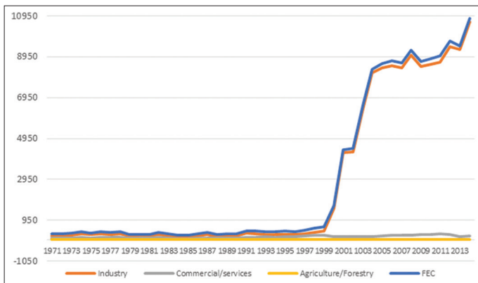
Graph 4: Final electricity consumption, by economic sector (GWh)
