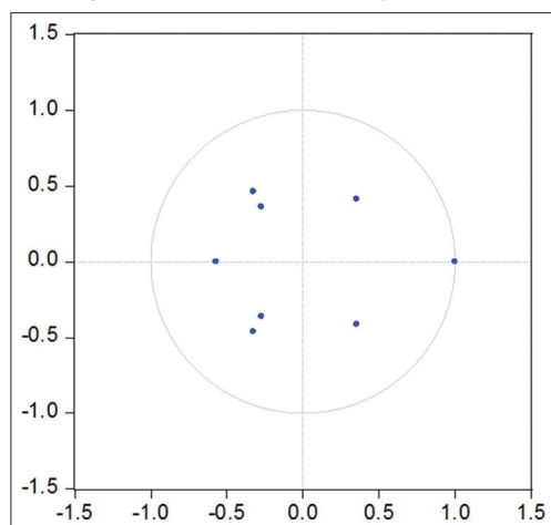
Figure 2: Inverse root stability test result
