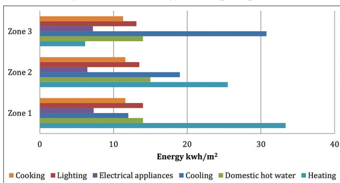
Figure 2: Annual energy consumption per area
