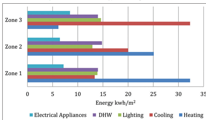
Figure 4: Annual energy consumption/ area
