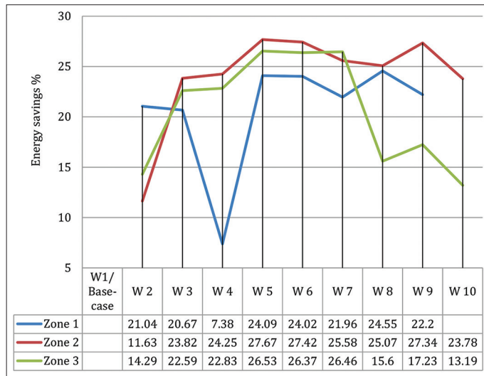
Figure 6: Energy saving of Wall systems alternatives
