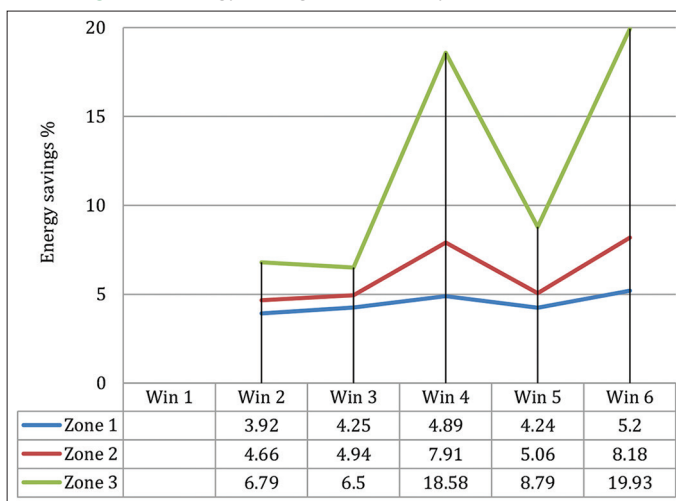
Figure 8: Energy saving of Window systems alternatives
