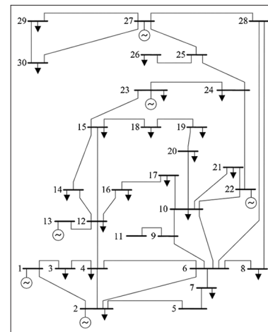
Figure 2: The IEEE 30-bus test system
