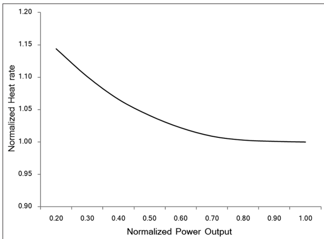
Figure 1: Output versus heat rate
