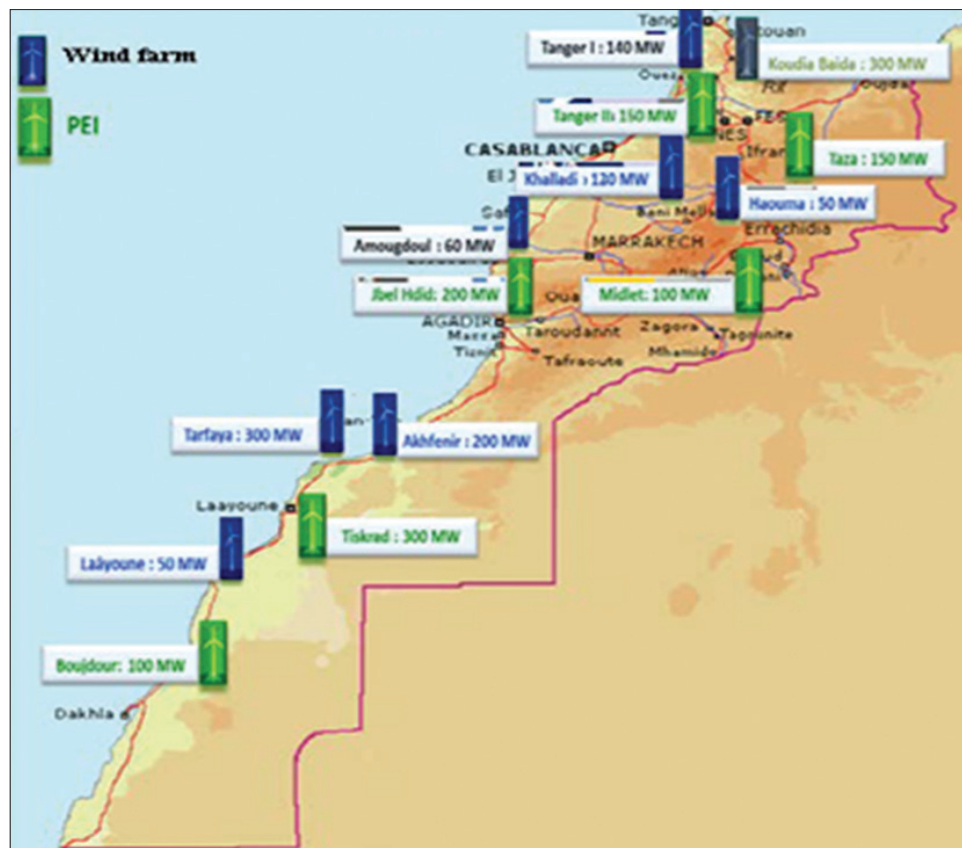
Figure 2: Morocco wind program. PEI: Integrated wind energy program
