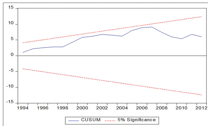
Figure 2: Cumulative sum of recursive residuals
