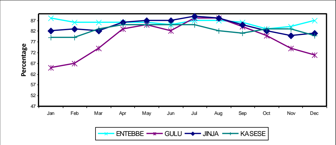
Figure 1.4 (c): Long term mean Relative Humidity at 06:00 hours for selected centres, 2016
