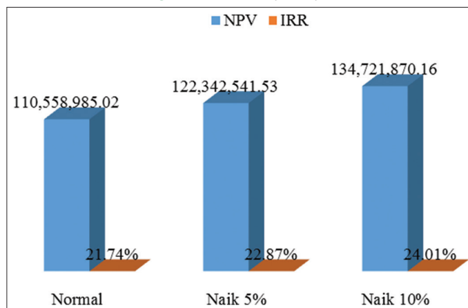
Figure 4: Sensitivity analysis
