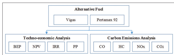
Figure 1: Research Methodology
