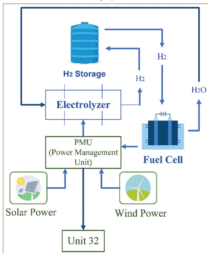
Figure 9: Schematic of the hybrid renewable energy with the hydrogen storage system
