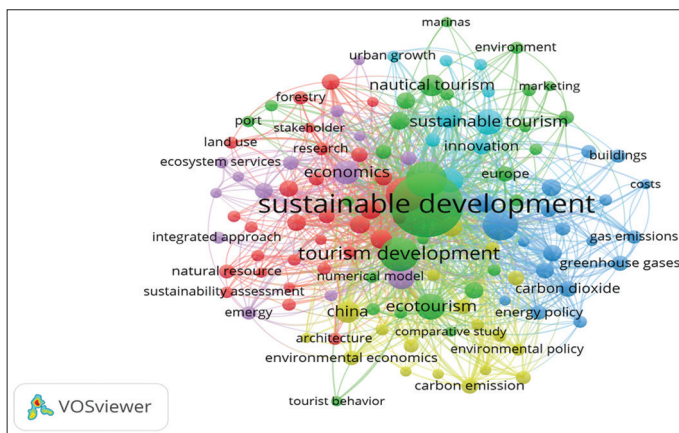
Figure 1: Keywords
