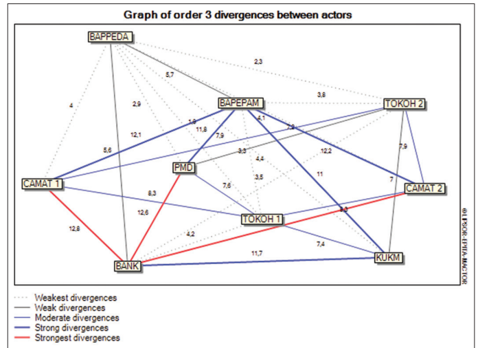
Figure 4: Order 3 divergence
