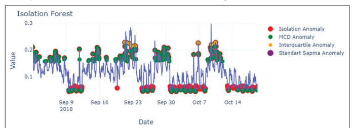
Figure 2: A view of extreme values for September-October, 2018
