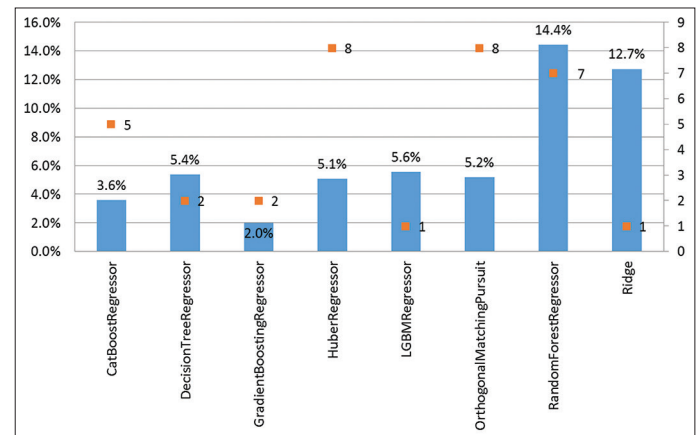
Figure 13: The frequencies of best performing methodologies
