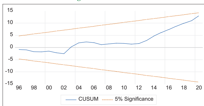
Figure 2: CUSUM test
