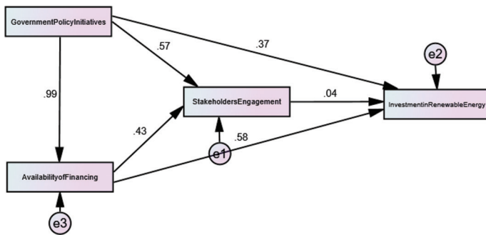
Figure 2: Standardized regression weights
