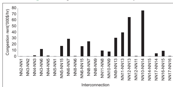
Figure 4: Congestion rent for the whole system
