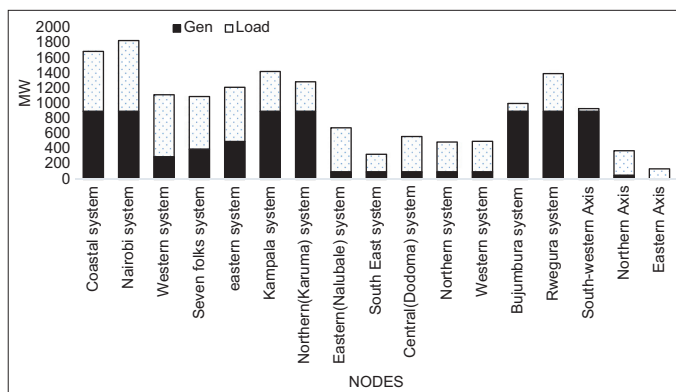
Figure 3: Comparison of generation and demand
