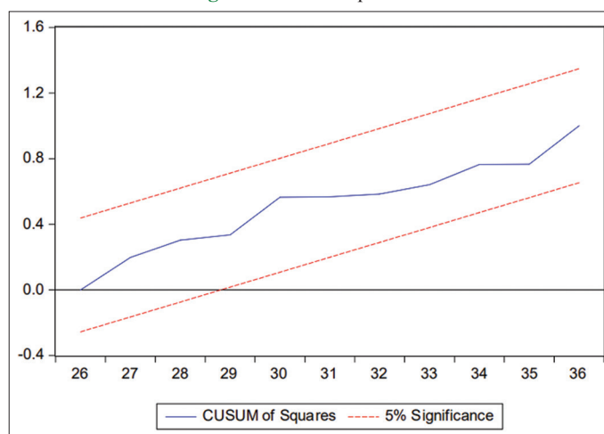
Figure 3: Cusum square test
