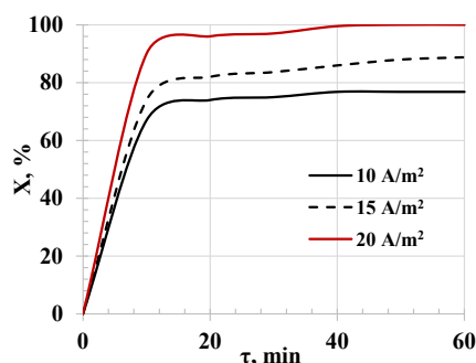
Fig. 3. Dependence of the degree of wastewater purification on the current density and duration of the process on aluminum anodes (Table 4)
