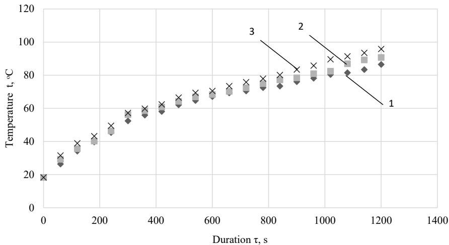
Fig. 9. The effect of layer thickness on the change in product temperature over time: 1 – 0.003 m; 2 – 0.005 m; 3 – 0.01 m
