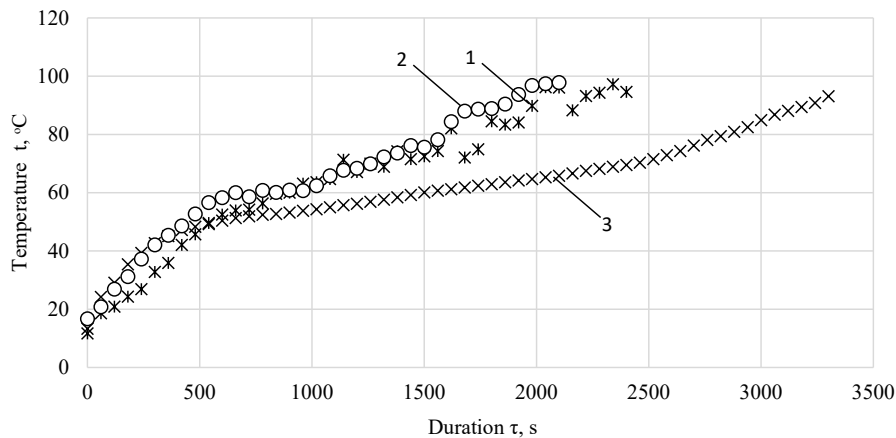
Fig. 7. Thermograms of slices of vegetables and fruits over time: 1 – carrot; 2 – apple; 3 – onion
