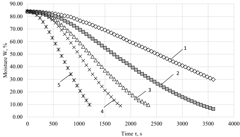
Fig. 2. The influence of the level of the supplied power of IR radiation on the change in product moisture content over time: 1 – 1.9 kW/m 2 ; 2 – 3.8 kW/m 2 ; 3 – 6 kW/m 2 ; 4 – 8.8 kW/m 2 ; 5 – 11.3 kW/m 2
