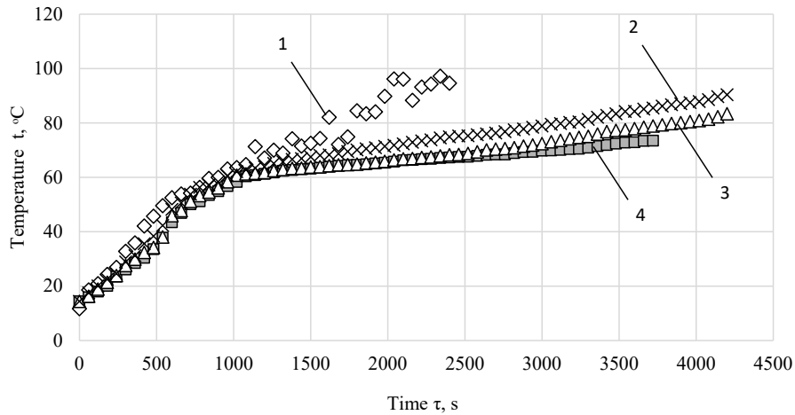
Fig. 5. The effect of layer thickness on the change in product temperature over time: 1 – 0.003 m; 2 – 0.005 m; 3 – 0.007 m; 4 – 0.01 m
