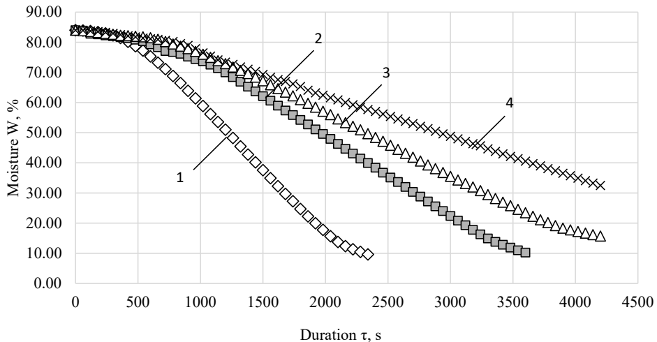
Fig. 4. The influence of the layer thickness on the change in product moisture over time: 1 – 0.003 m; 2 – 0.005 m; 3 – 0.007 m; 4 – 0.01 m
