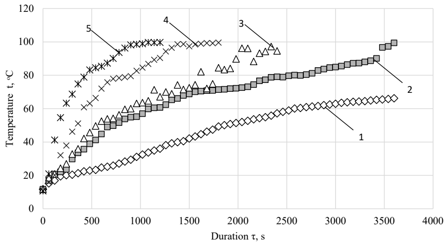
Fig. 3. The influence of the level of the supplied power of IR radiation on the change in the temperature of the product over time: 1 – 1.9 kW/m 2 ; 2 – 3.8 kW/m 2 ; 3 – 6 kW/m 2 ; 4 – 8.8 kW/m 2 ; 5 – 11.3 kW/m 2
