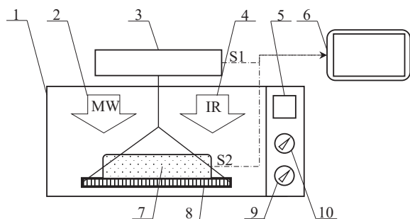
Fig. 1. Scheme of a universal stand for researching drying processes in electromagnetic fields: 1 – drying chamber; 2 – MW generator; 3 – electronic scales; 4 – IR generator; 5 – time table; 6 – data collection and payment system; 7 – vegetable raw materials; 8 – cassette; 9 – power regulator of the MW generator; 10 – IR generator power regulator; S1 – signal from electronic scales; S2 – temperature sensor signal
