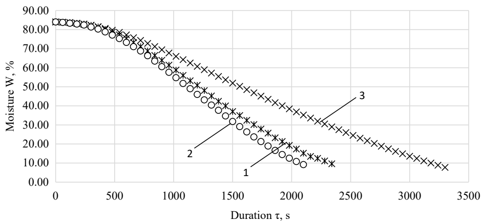
Fig. 6. Changes in moisture content of slices of vegetables and fruits over time: 1 – carrot; 2 – apple; 3 – onion
