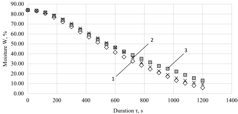
Fig. 8. The influence of the layer thickness on the change in product moisture over time: 1 – 0.003 m; 2 – 0.005 m; 3 – 0.01 m
