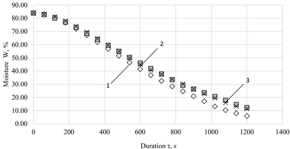
Fig. 10. Change in moisture of slices of vegetables and fruits over time: 1 – carrot; 2 – apple; 3 – onion
