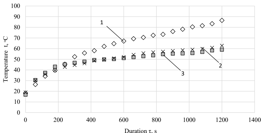
Fig. 11. Thermograms of slices of vegetables and fruits over time: 1 – carrot; 2 – apple; 3 – onion
