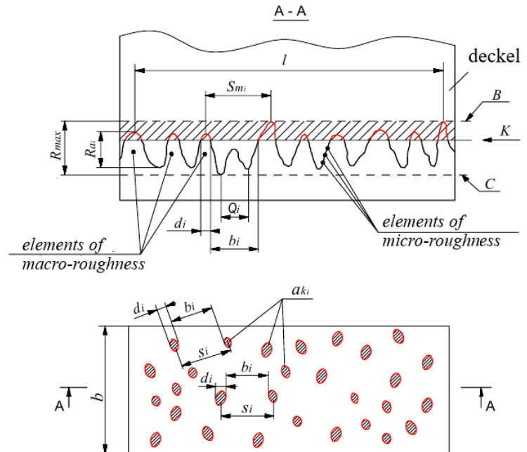
Fig. 1. Scheme of recesses of micro protrusions of the roughness of the surface of the printing plate: K – plane of contact of the deckel surface with the elements of the macro-roughness of the printing plate; C – the plane of the largest depressions of the macro-roughness profile in the deckel contact zone; B – the plane of the largest microprotrusions of the macro-roughness profile in the deckel contact zone; l – base length, mm; b and L – respectively, the width and length of the contact zone between the plate and offset cylinders, mm; S_i – the pitch of local protrusions, \mu\text{m} ; S_{mi} – the step between the protrusions of the deckel contact with the surface of the printing plate within the base length, microns; R_{ai} – the partial depth of the roughness troughs, which is the vertical distance between the adjacent top and bottom of the roughness element, \mu\text{m} ; d_i – the microprotrusion imprint diameter, \mu\text{m} ; b_i – the distance between the imprints of microprotrusions, \mu\text{m} ; Q_i – the pitch of adjacent roughness microcavities, \mu\text{m} ; a_{ki} – spot area
