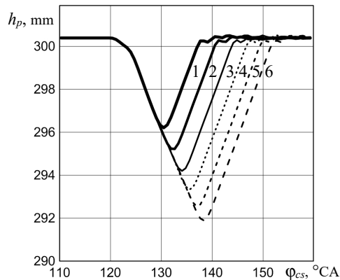
Fig. 2. Dependence of the stroke metering piston on the angle of rotation the crankshaft: 1 – \varphi_v = 6.6 °CA; 2 – \varphi_v = 8.4 °CA; 3 – \varphi_v = 10.2 °CA; 4 – \varphi_v = 12 °CA; 5 – \varphi_v = 13.2 °CA; 6 – \varphi_v = 14.4 °CA
