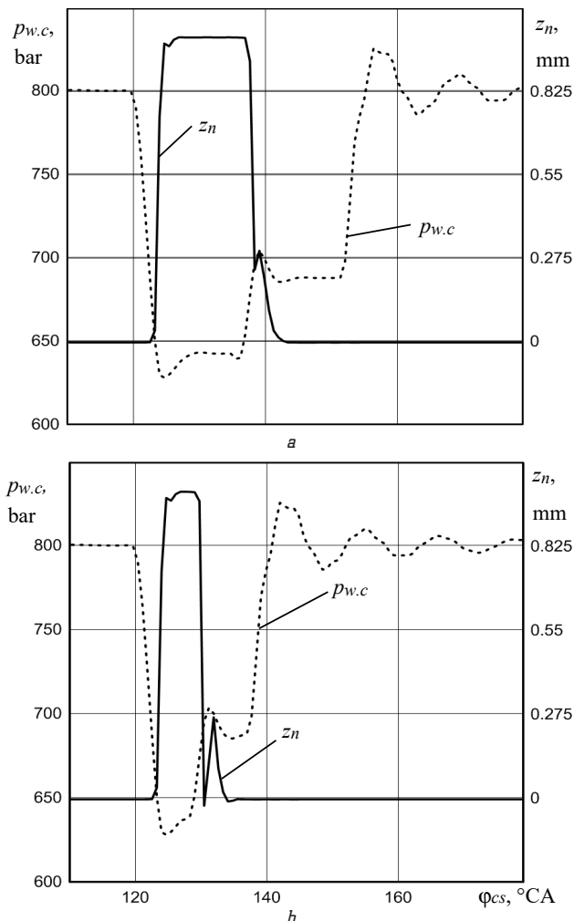
Fig. 5. Oscillograms of injector operation at: a – \varphi_v=14.4 °CA; b – \varphi_v=6.6 °CA; z_n – stroke of the nozzle needle; p_{w.c} – pressure in the working cavity of the ICU
