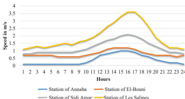
Fig. 2. Wind speed average hourly profile in Annaba province
