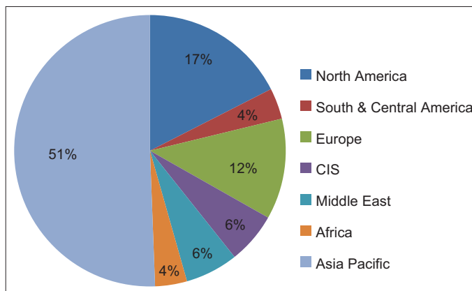
Figure 1: Contribution of CO 2 Emissions in Different Groups of Countries to the World in 2020
