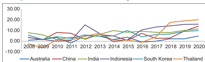
Figure 5: Growth of environmental degradation in Asia Pacific
