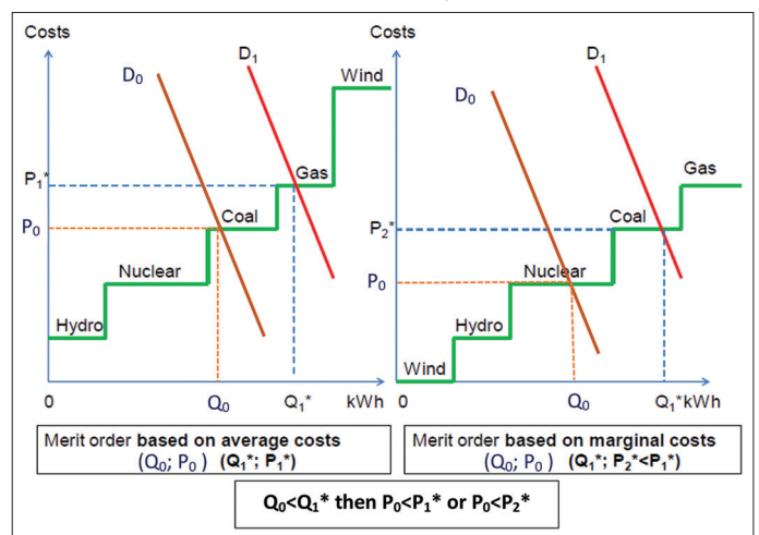
Figure 1: The cost of the electricity system in order to answer the evolution of electricity demand
