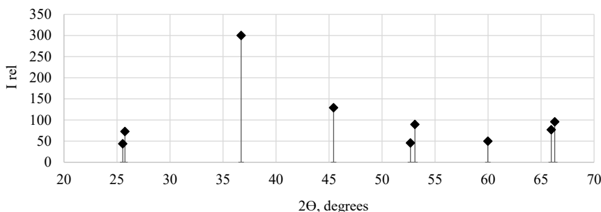
Fig. 1. Radiograph of the ceramic mass of barium titanate fired at temperature 1350 °C: ◆ – BaTiO 3
