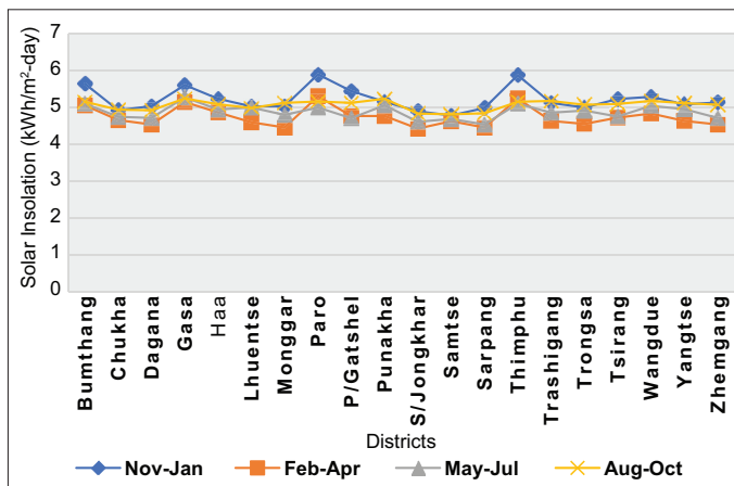
Figure 2: Seasonal solar insolation at latitude tilt by district
