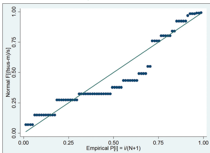
Figure 1: Outliers
