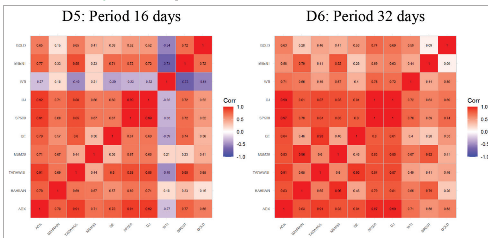
Figure 2: Decomposed correlation at resolution levels D5 and D6
