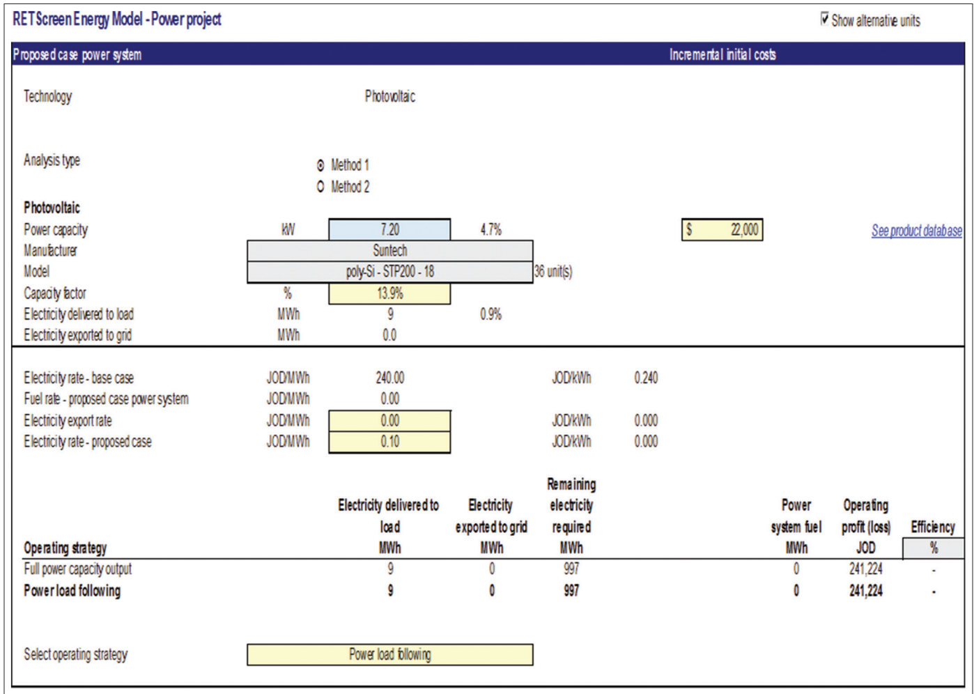
Figure 8: Power system (Proposed case) for Netherland embassy project
