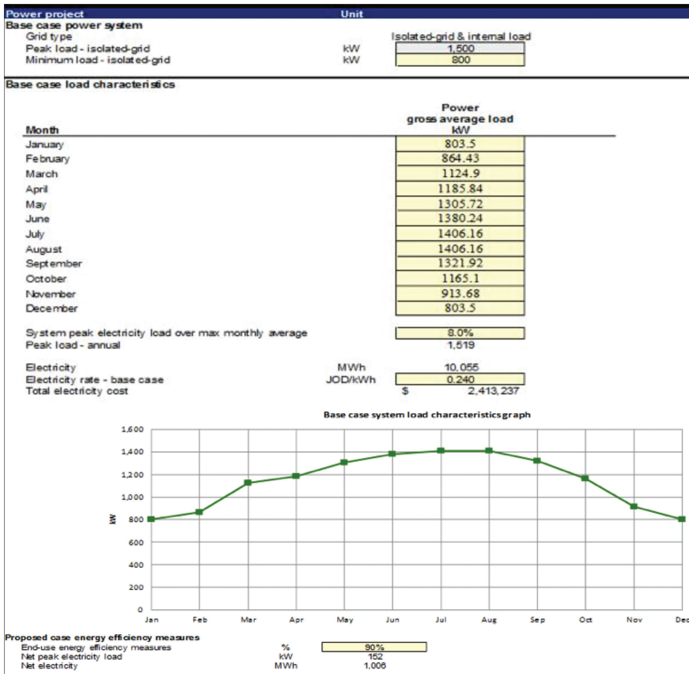
Figure 10: Base case power system of the embassy project
