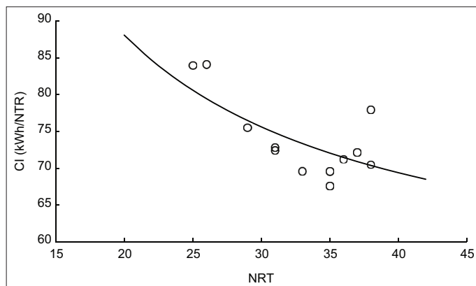
Figure 9: Electric energy consumption index
