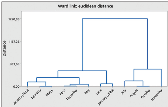
Figure 8: Dendrogram
