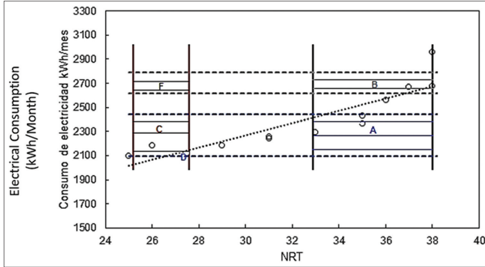
Figure 7: Intersection of points of high concentration of operations and of energy consumption
