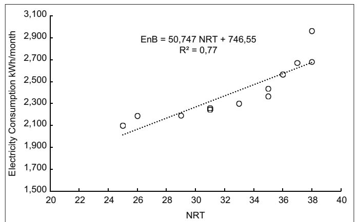
Figure 4: Electric energy baseline (EnB)
