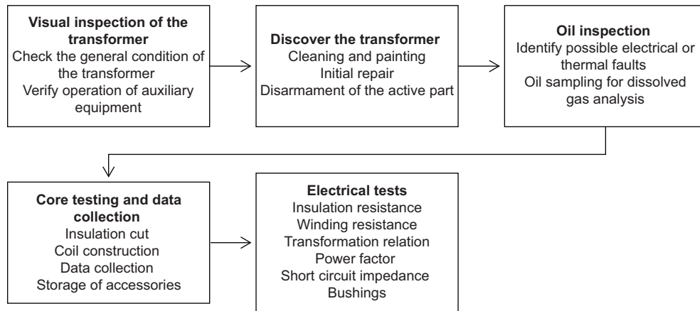
Figure 2: General transformer maintenance process
