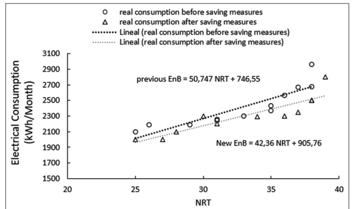
Figure 10: New electricity consumption baseline (EnB)
