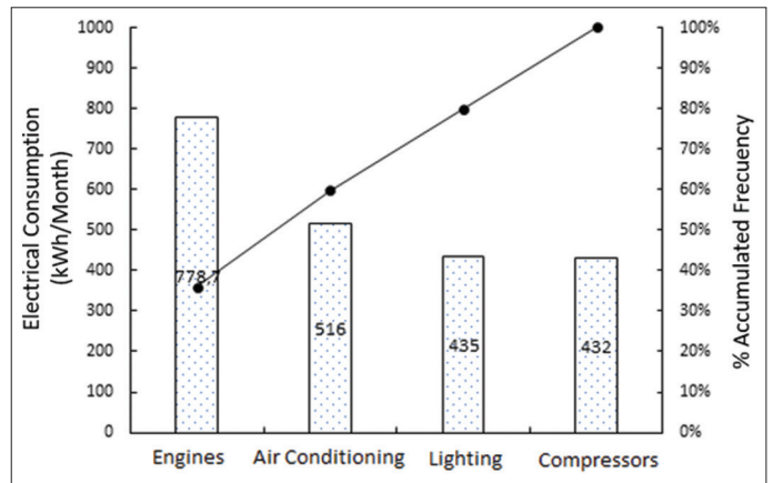
Figure 3: Pareto diagram on energy consumption by the company’s equipment
