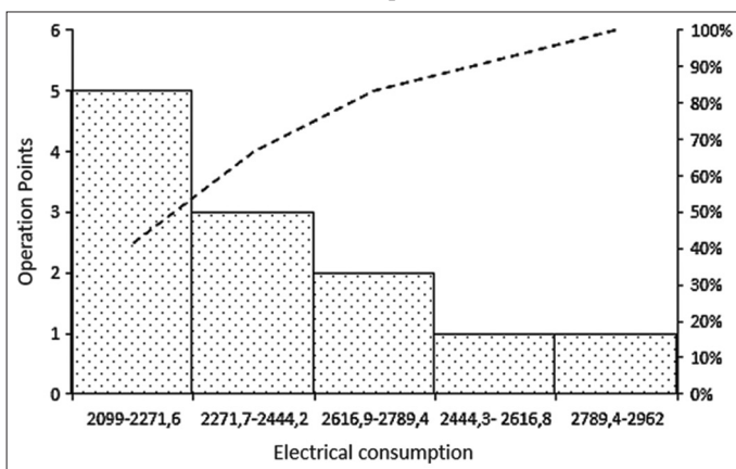
Figure 6: Pareto of operating points in terms of electricity consumption
