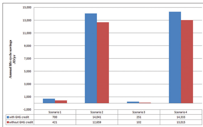
Figure 6: Annual cycle saving for different scenarios for the commercial and hotels electricity tariff
