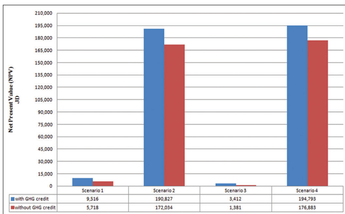
Figure 5: The net current value for different scenarios for the commercial and hotels electricity tariff
