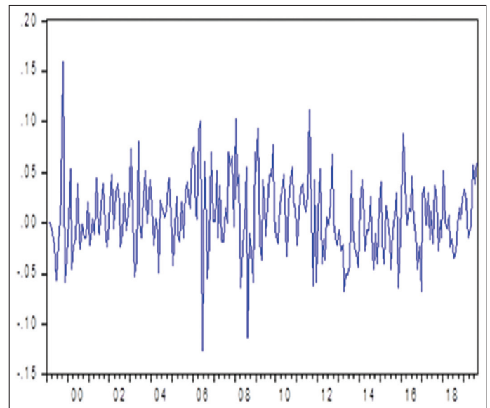
Figure 3: Graphical representation of the first difference series DLNGP
