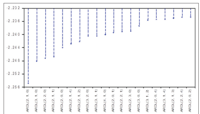
Figure 4: Results of AIC-based appropriate lag periods test
