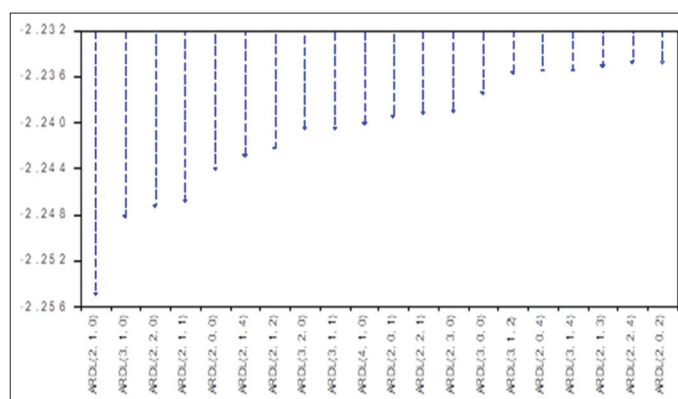
Figure 4: Results of AIC-based appropriate lag periods test
