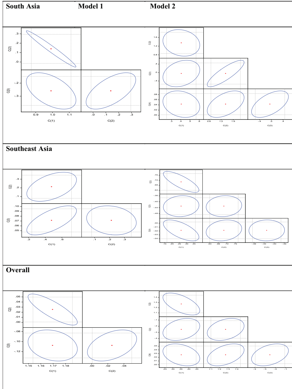
Figure 1: Coefficient diagnostics confidence interval (ellipse test)
