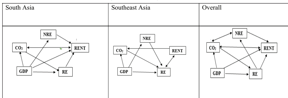
Figure 2: Causality directions
