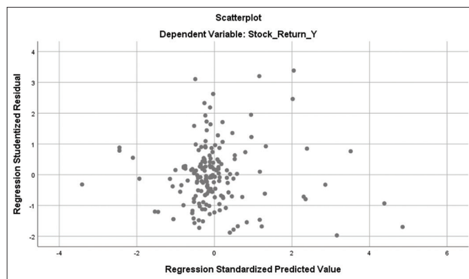
Figure 2: Heteroskedasticity test
