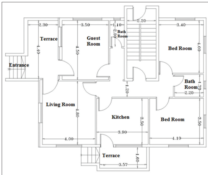
Figure 1: Floor plan of the selected houses
