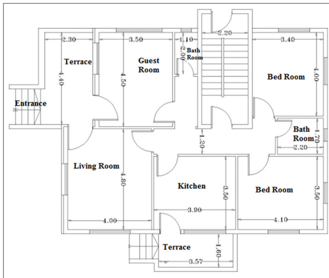
Figure 1: Floor plan of the selected houses
