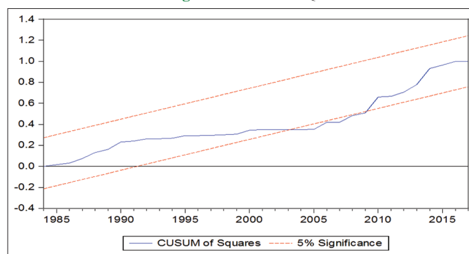
Figure 4: CUSUMSQ
