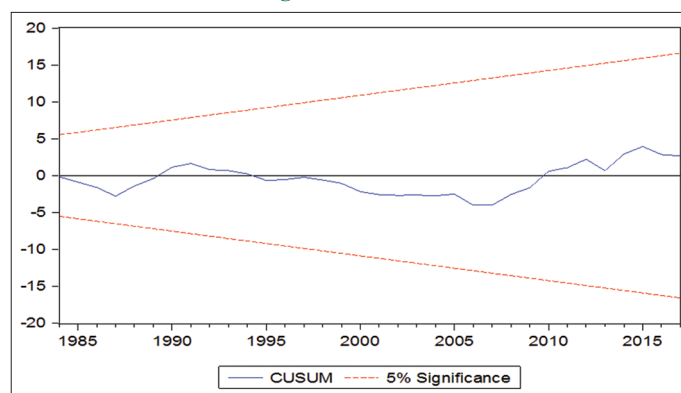
Figure 3: CUSUM
