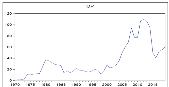
Figure 1: Oil Prices (1970-2019)
