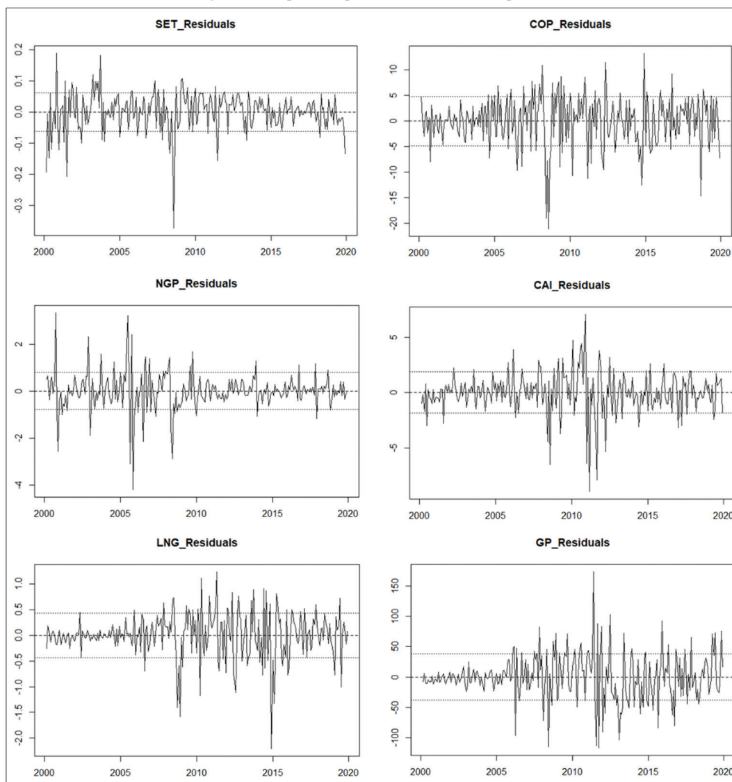
Figure 1: Graphical representation of variable proxies
