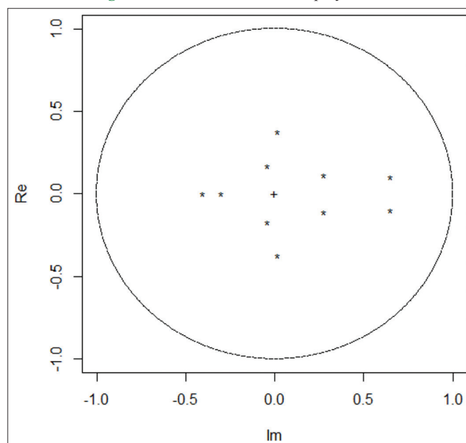
Figure 2: Roots of characteristic polynomial
