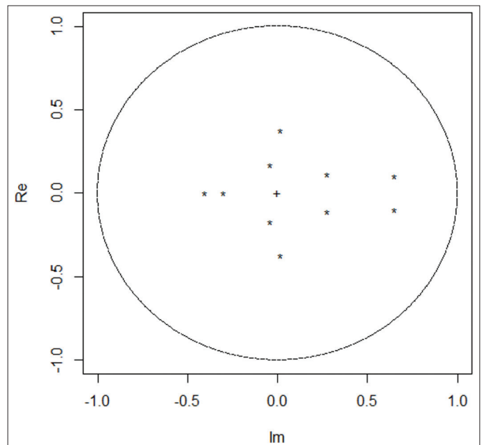
Figure 2: Roots of characteristic polynomial
