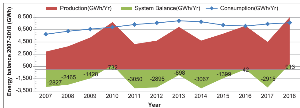
Figure 1: Historical electricity balance in Albania, 2007-2018 (ERE, 2018)
