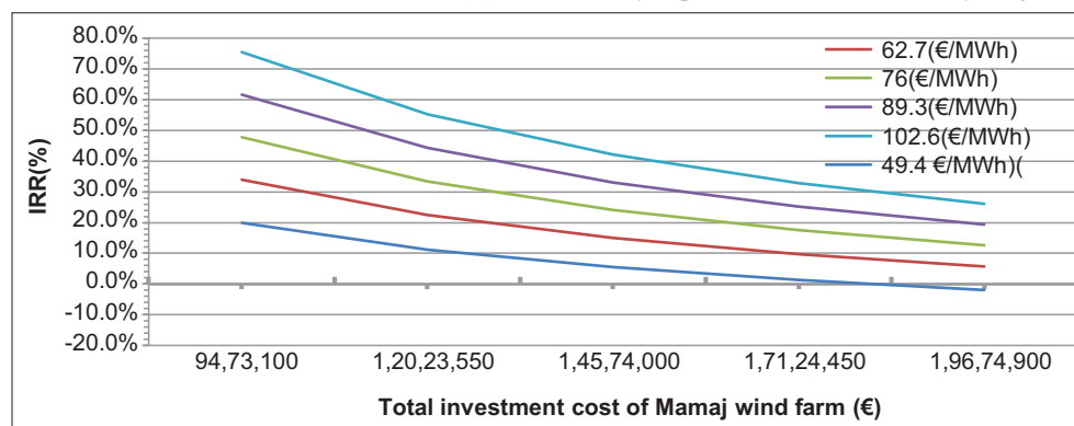
Figure 13: IRR variation as a function of total investment cost (€) and electricity export rate within a sensitivity range of (\pm 35)\% , r = (5\div 11)\% .
