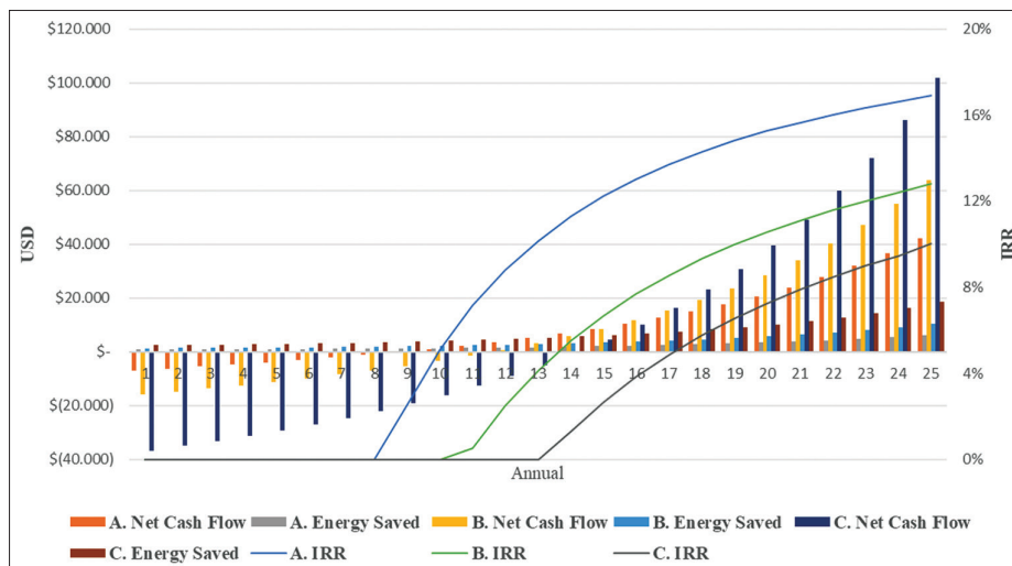
Figure 8: Financial comparison of generation scenarios (HIT)
