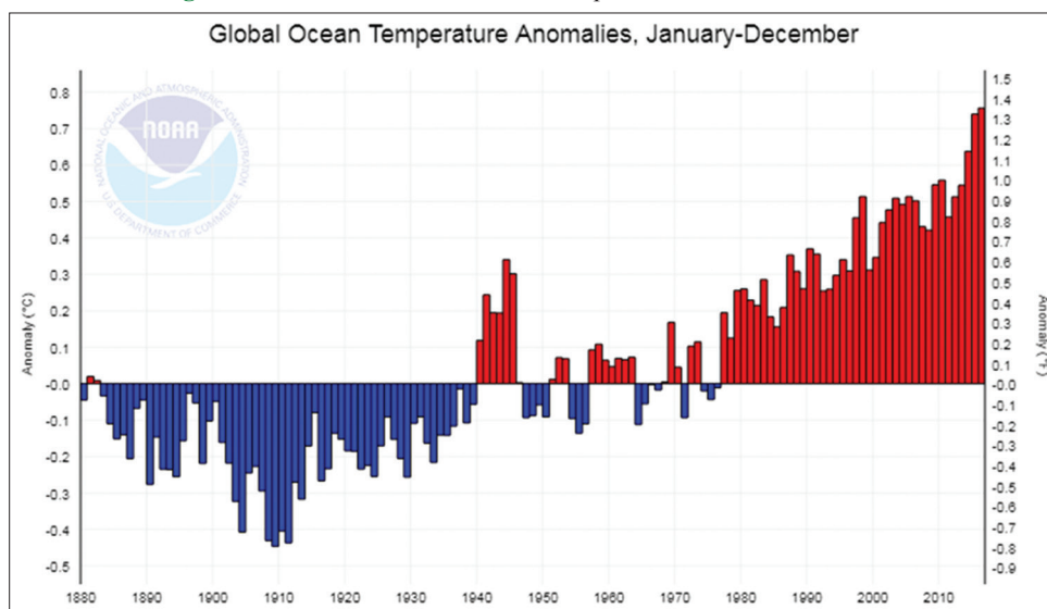
Figure 11: Global annual sea surface temperature anomalies from 1880 to 2016
