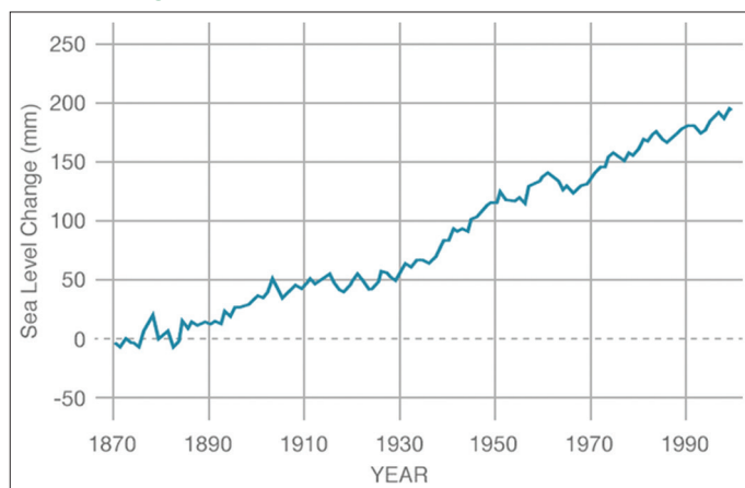
Figure 13: Global mean sea level rise anomalies
