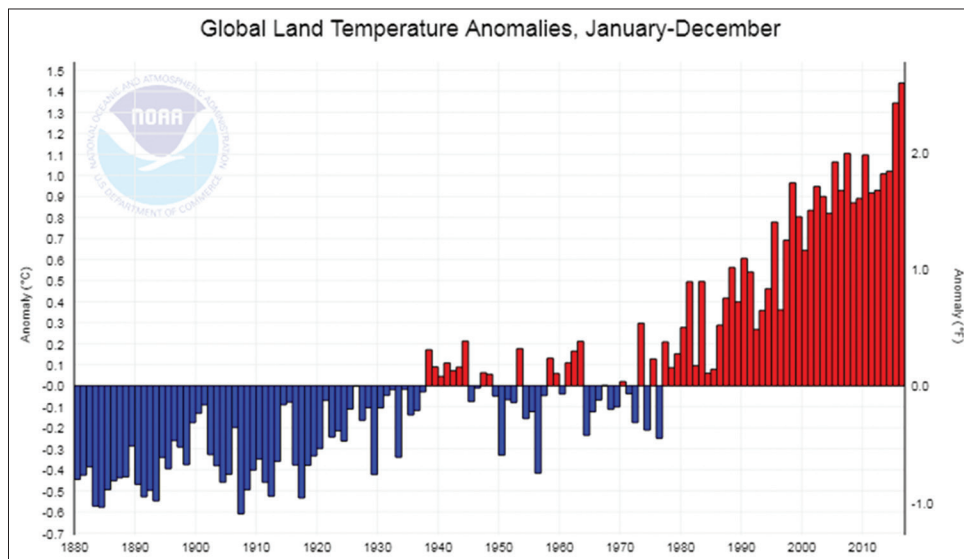
Figure 9: Global annual land surface air temperature anomalies from 1880 to 2016
