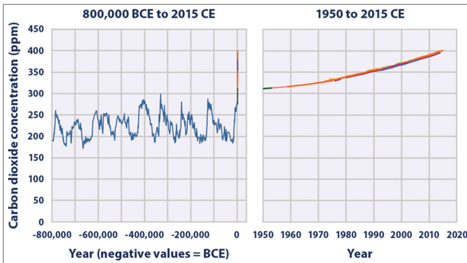
Figure 2: Carbon dioxide concentration since last 800,000 years (left hand side) and since 1950 (right hand side)
