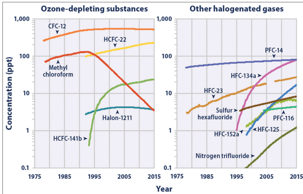
Figure 5: Halo carbon concentration since 1975
