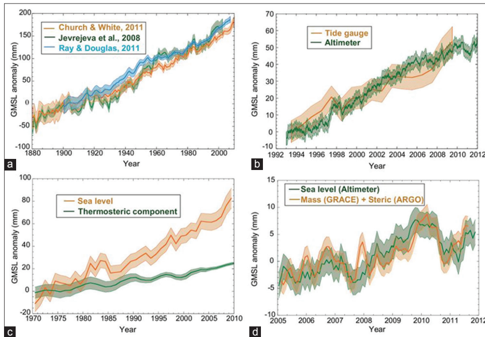
Figure 12: (a-d) Global mean sea level rise anomalies
