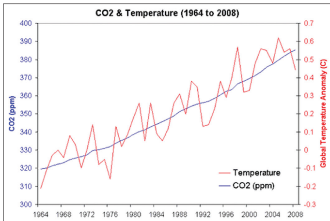
Figure 7: Statistical method of finding the relationship between greenhouse gases and Temperature shows that there is no correlation between these two variables. The CO 2 continues to rise, but there is a variation in the temperature
