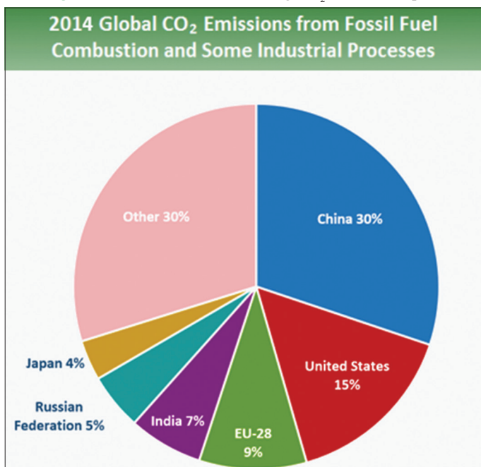
Figure 6: Global countries releasing CO 2 in the atmosphere
