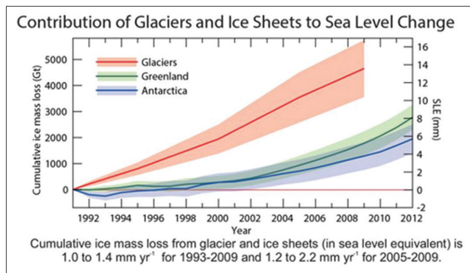
Figure 17: The ice mass loss equivalent to sea level from the Greenland and Antarctica
