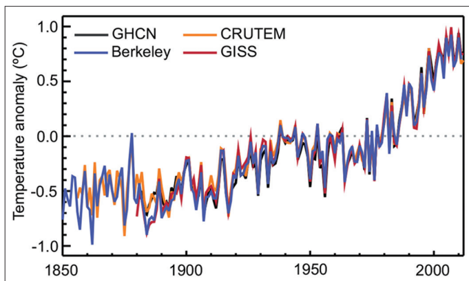
Figure 8: Global annual land surface air temperature anomalies. From 1961 to 1990 taken as an average
