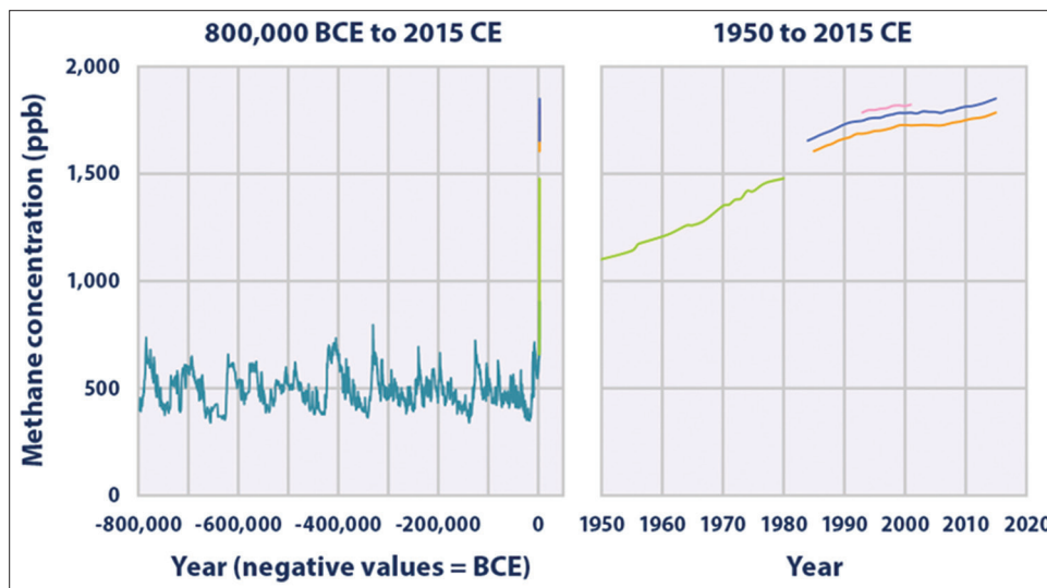
Figure 3: Methane concentration since last 800,000 years (left hand side) and since 1950 (right hand side)
