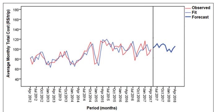
Figure 7: Observed monthly average total cost per trip in the period April 2012-2017 and forecast monthly average total cost per trip for the period of May 2017-April 2018
