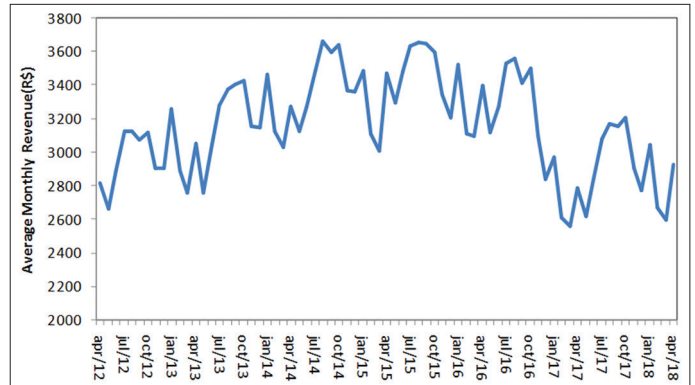
Figure 6: Observed monthly average revenue for the period April 2012-2017 and forecast monthly average income for the period May 2017-April 2018
