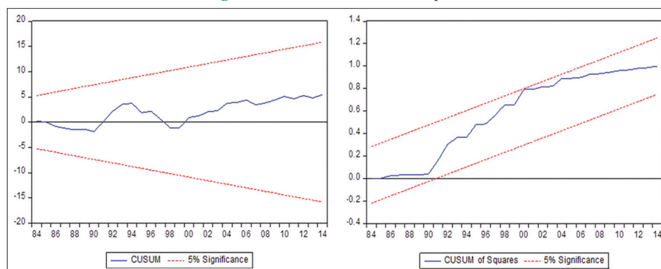
Figure 1: CUSUM and CUSUMsq tests
