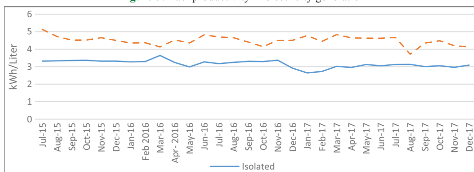
Figure 3: Fuel productivity in electricity generation
