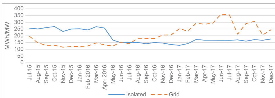
Figure 2: Capital productivity in electricity generation
