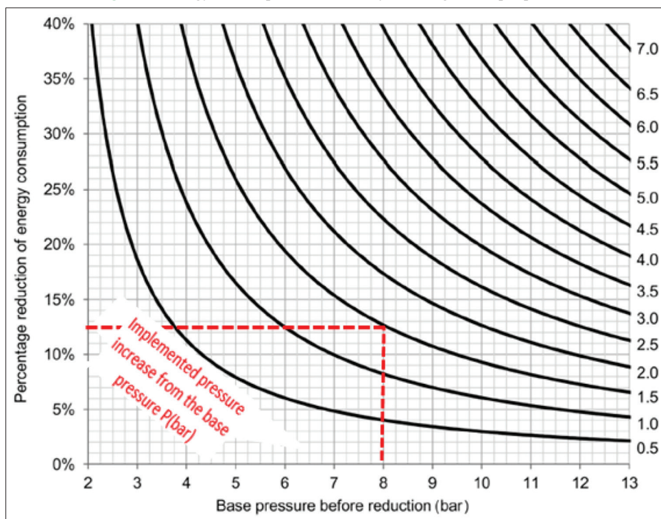
Figure 5: Energy consumption reduction by lowering the output pressure
