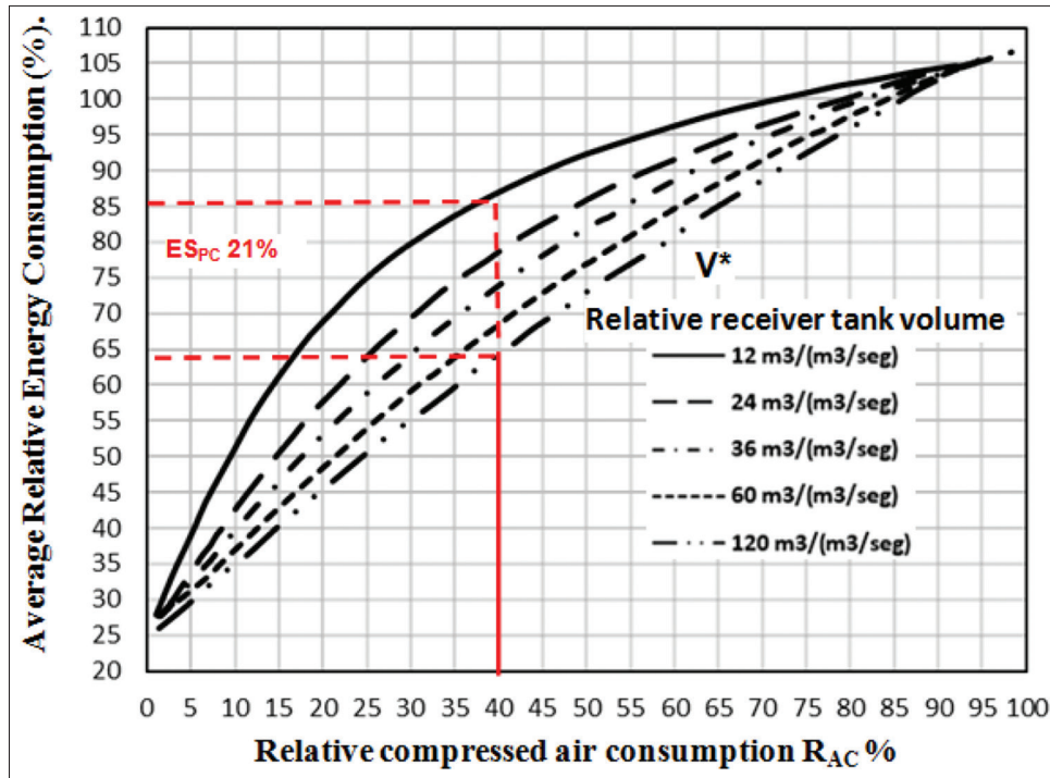
Figure 4: Relative energy consumption for different relative receiver tank volumes as a function of relative compressed air consumption
