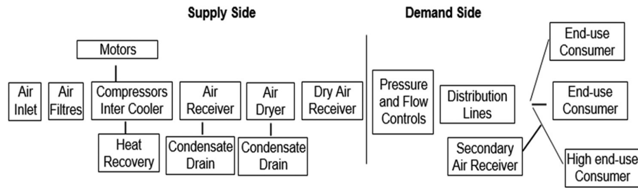
Figure 3: CAS and elements divided according to supply and demand sides
