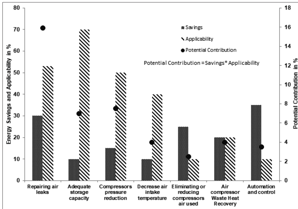
Figure 6: Energy saving, applicability and potential of contribution for different improvement measures in CASs
