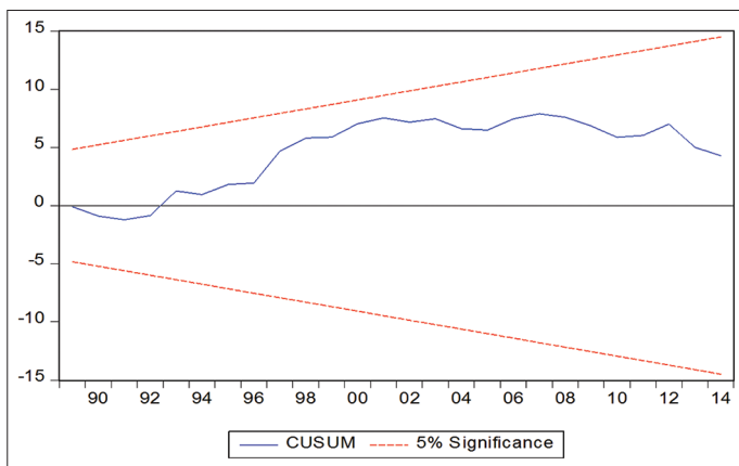
Figure 1: Cumulative sum of recursive residual
