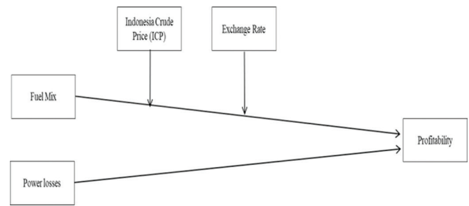
Figure 1: Research model
