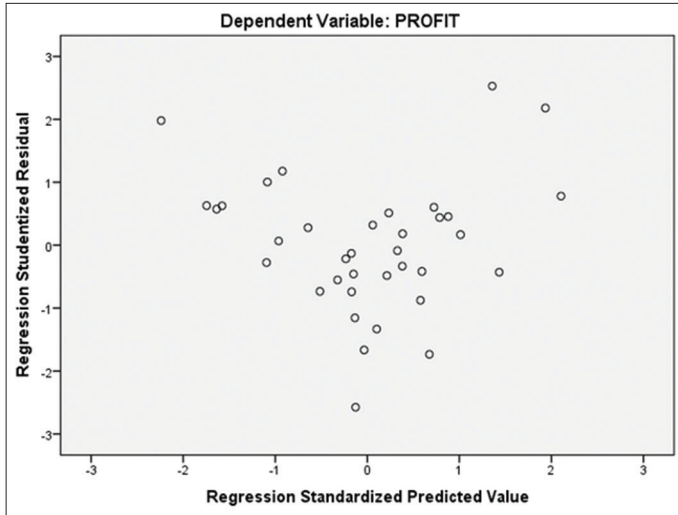
Graph 1: Scatterplot diagram as heterokedasticity test output
