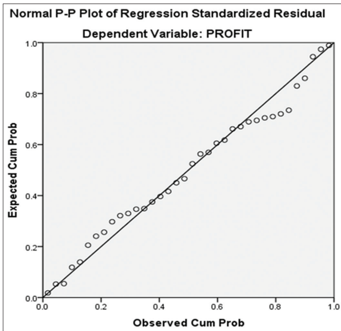
Graph 2: P-Plot diagram as normality test output
