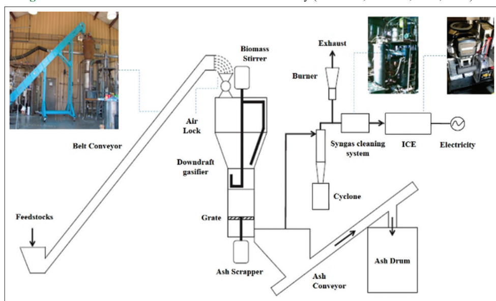
Figure 3: Schematics of the 60kW ICDG used in this study (Indrawan, Simkins, et al., 2020)
