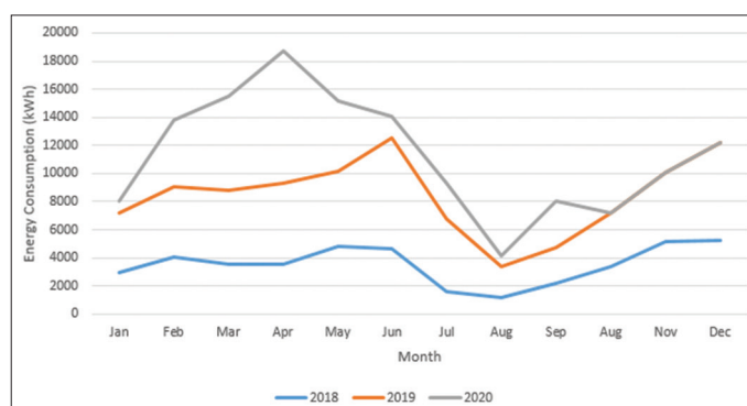
Figure 2: Monthly load profile of the Odum block (based on data obtained from NEDCo)
