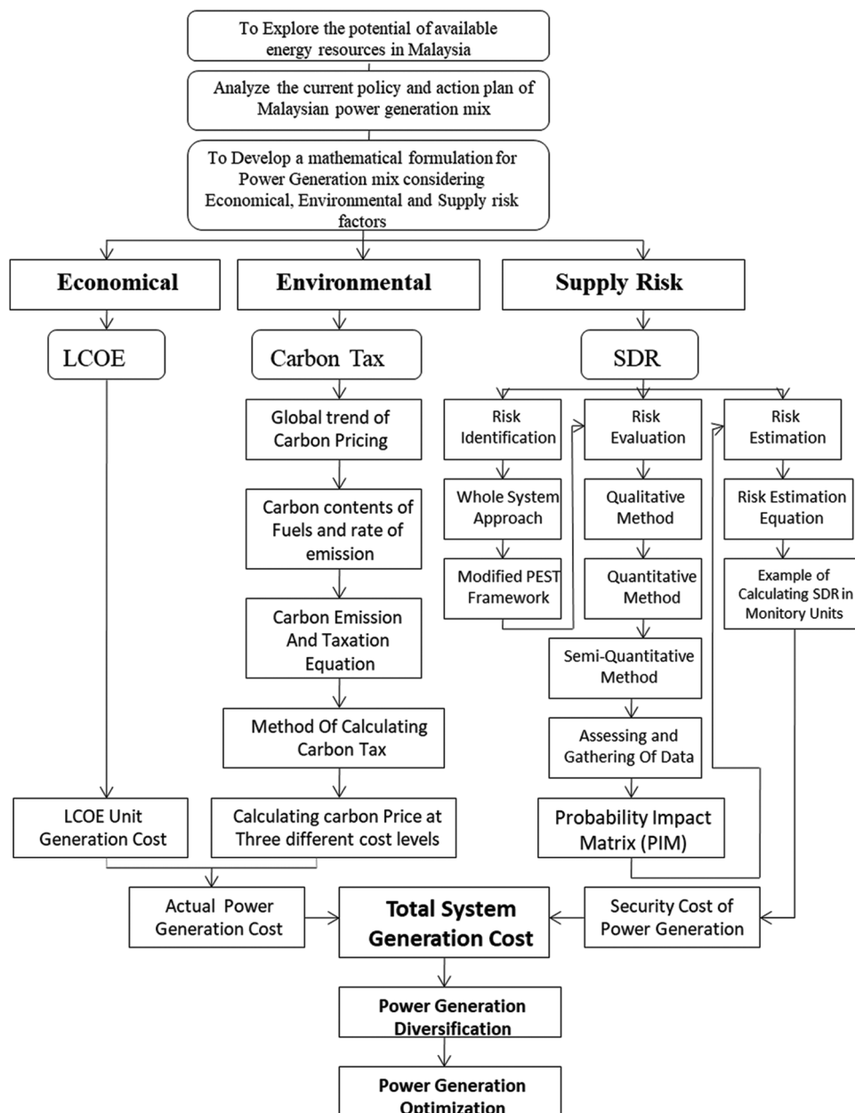
Figure 2: Research framework
