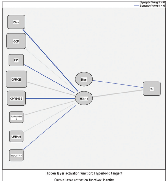
Figure 1: Neural network architecture
