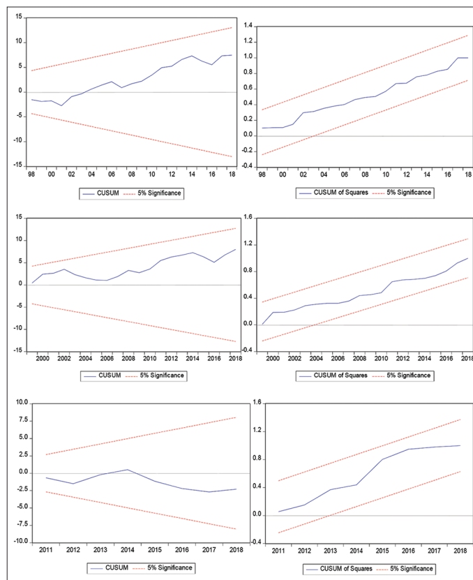
Figure 4: CUSUM and CUSUM squares stability test
