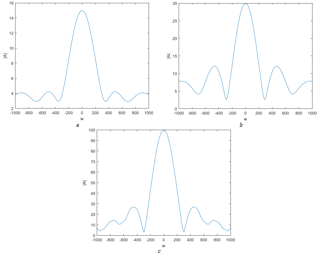
Fig. 2. Results of numerical simulation |A_2(w)| for the Gaussian distribution of the probability density p(\Delta t) , due to a random phase shift in the range from -0.01 to 0.01 s, with the number of motor units: a - K=15 ; b - K=30 ; c - K=100
